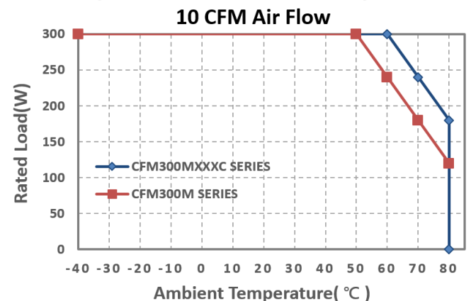
Output Power vs. Ambient Temperature 10 CFM Air Flow
